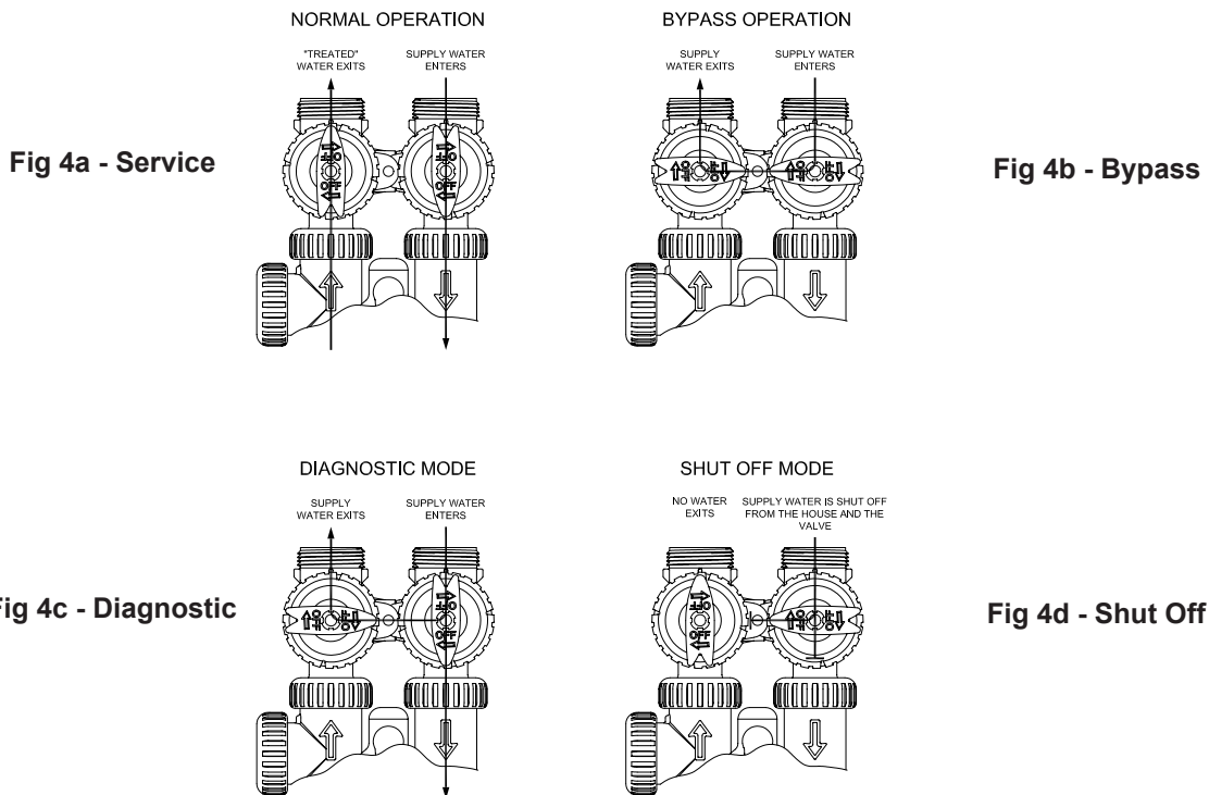
Figure 4: Bypass Valve Operation
