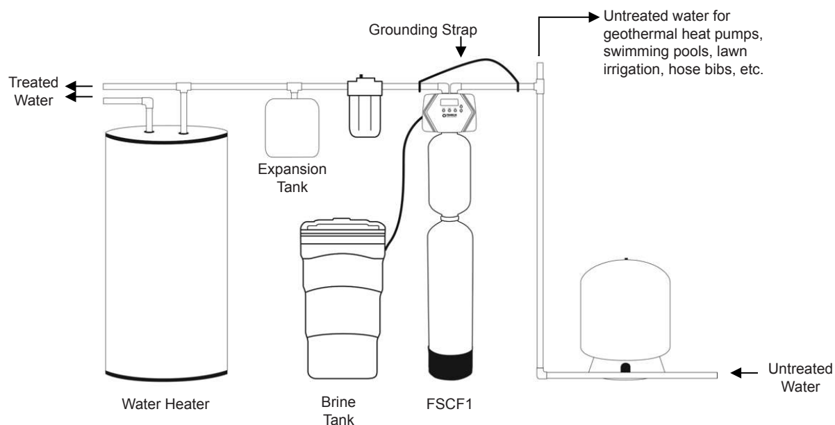
Figure 1: Typical Installation
