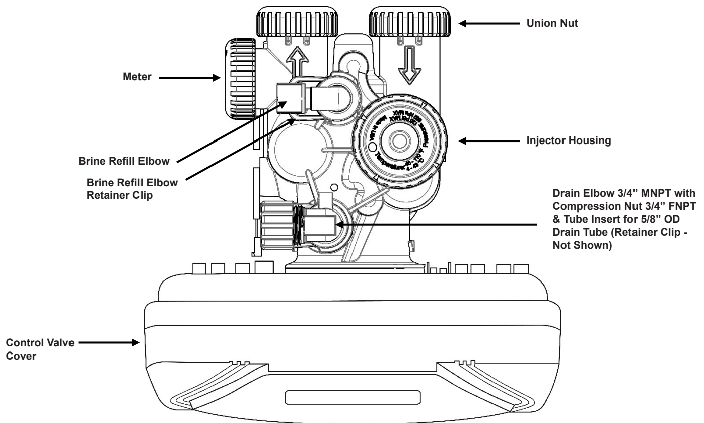
Figure 2: Top View of Control Valve
