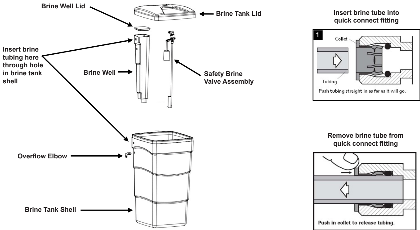
Figure 3: Brine Tank Components
